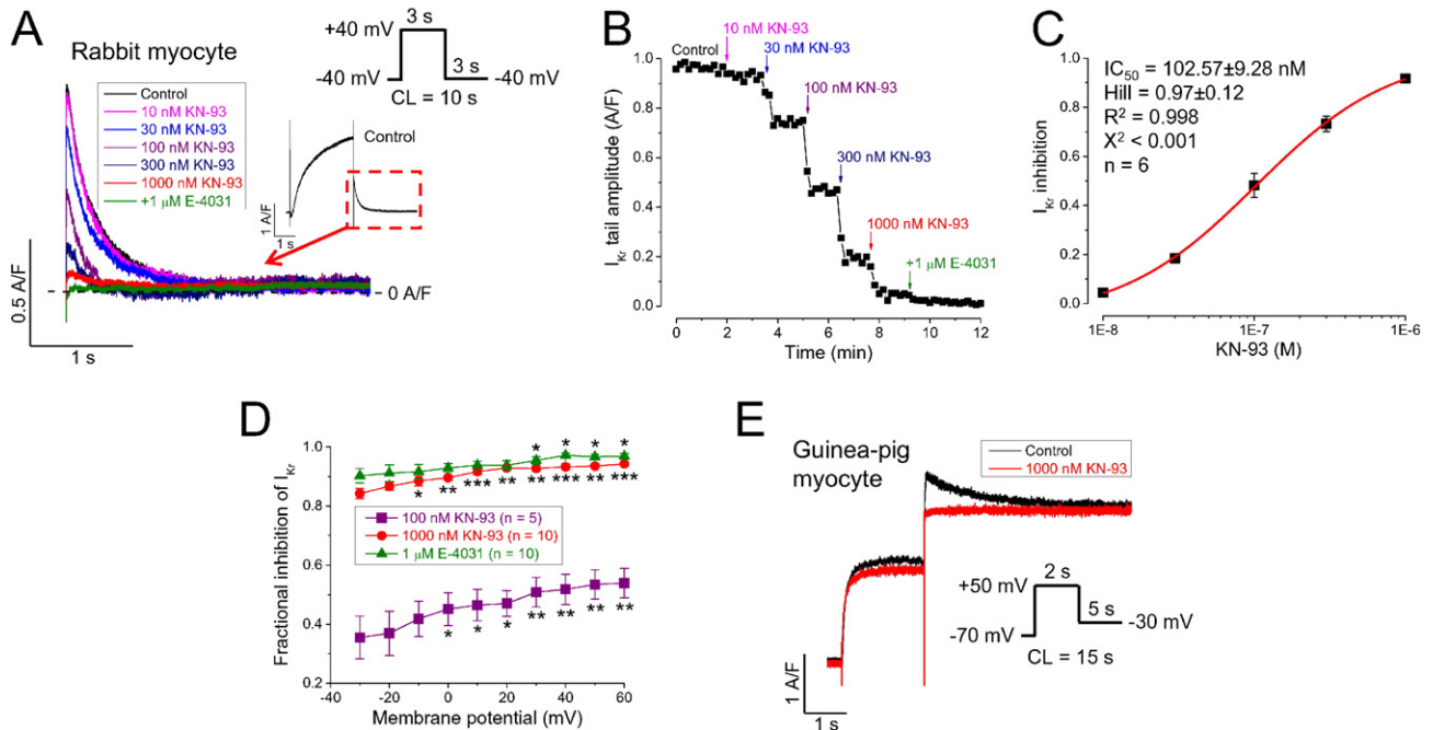
Fig. 2. KN-93 inhibits I_{Kr} in mammalian ventricular myocytes. Panel A: Concentration-dependent inhibition of I_{Kr} in rabbit ventricular myocytes measured as tail current under conventional voltage clamp conditions with 10 mM BAPTA in the pipette solution. Panel B: Time course of the development of the effect of KN-93 on I_{Kr} recorded in a representative cell. Note that the inhibitory effect develops within 1 min and KN-93 abolished completely the E-4031 sensitive current. Panel C: Dose response curve obtained from 6 ventricular cells. Panel D: KN-93 inhibits I_{Kr} at all membrane potentials but the inhibition is more effective at positive voltages. Asterisks indicate significant differences from fractional inhibition measured at -30 mV (*: p < 0.05 , **: p < 0.02 , ***: p < 0.001 ). Panel E: Representative superimposed current traces recorded before and after the administration of 1 \mu M KN-93 in guinea pig ventricular myocyte with the voltage command shown in the inset. KN-93 abolished the tail current indicating complete inhibition of I_{Kr} .
